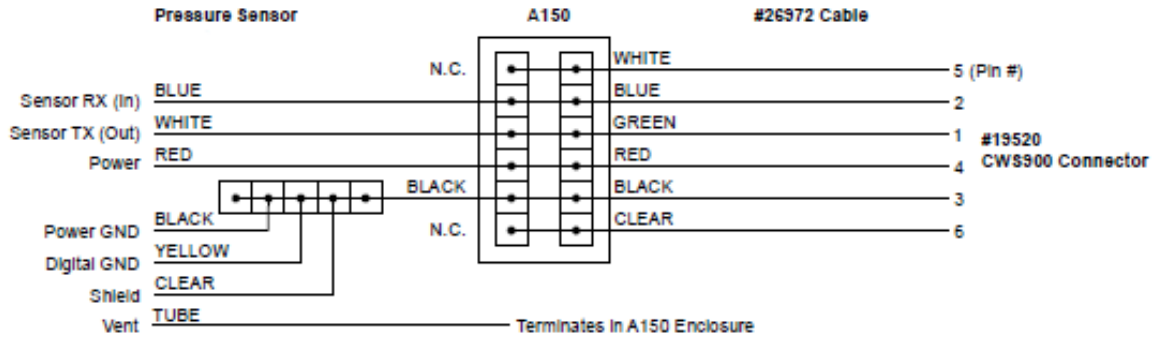
FIGURE 7-4. A150 wired for CS451 pressure sensor and CWS900 connector
